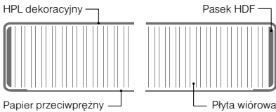
Profile U-U R = 3.3 mm
